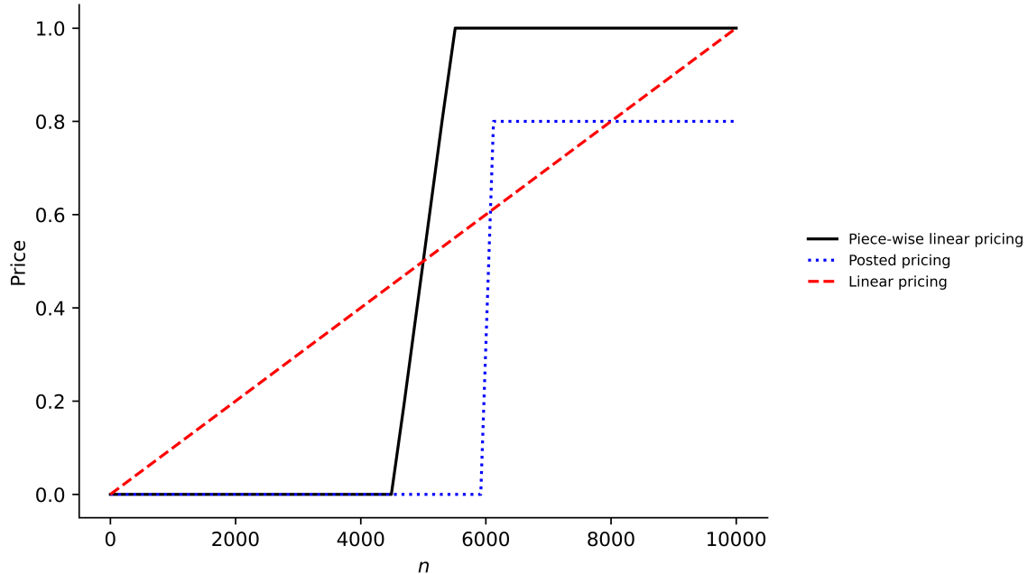
Figure 1: Pricing rules.
