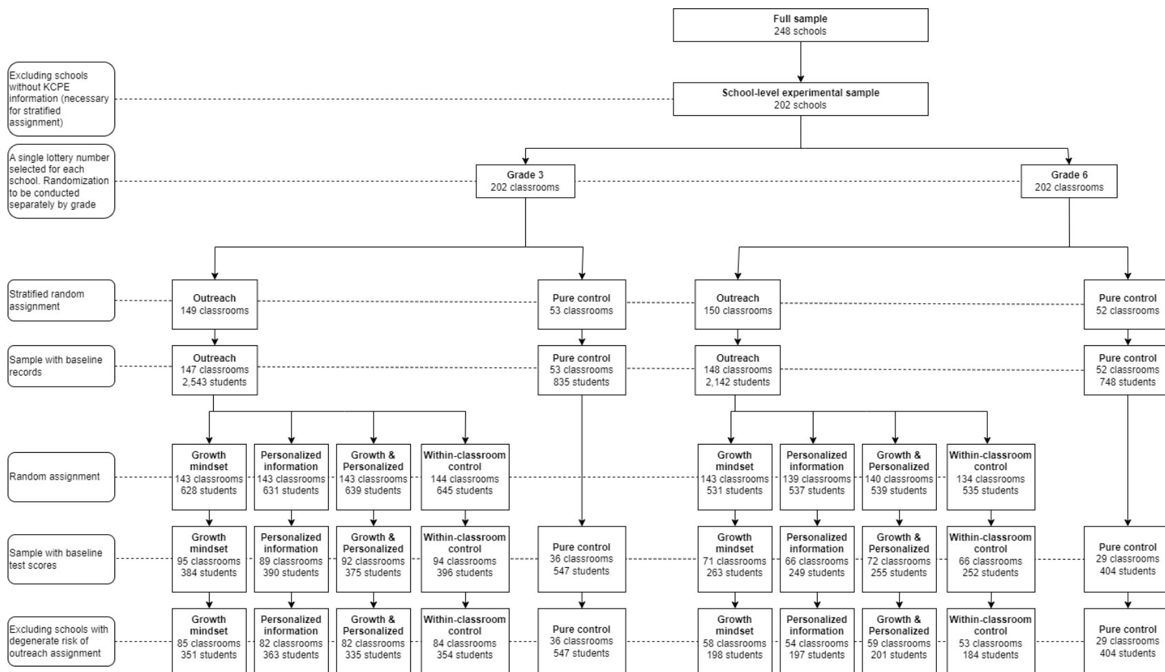
Figure 2: Consort diagram
