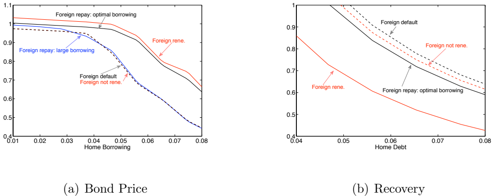
Figure 2: Equilibrium Functions
