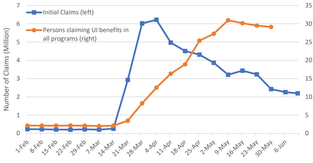
Figure 4: Numbers of UI Weekly Claims
