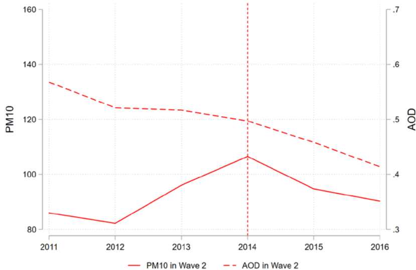
(B) Wave 2 Cities: PM 10 and AOD
