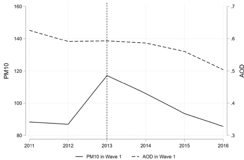
(A). Wave 1 Cities: PM_{10} and AOD
