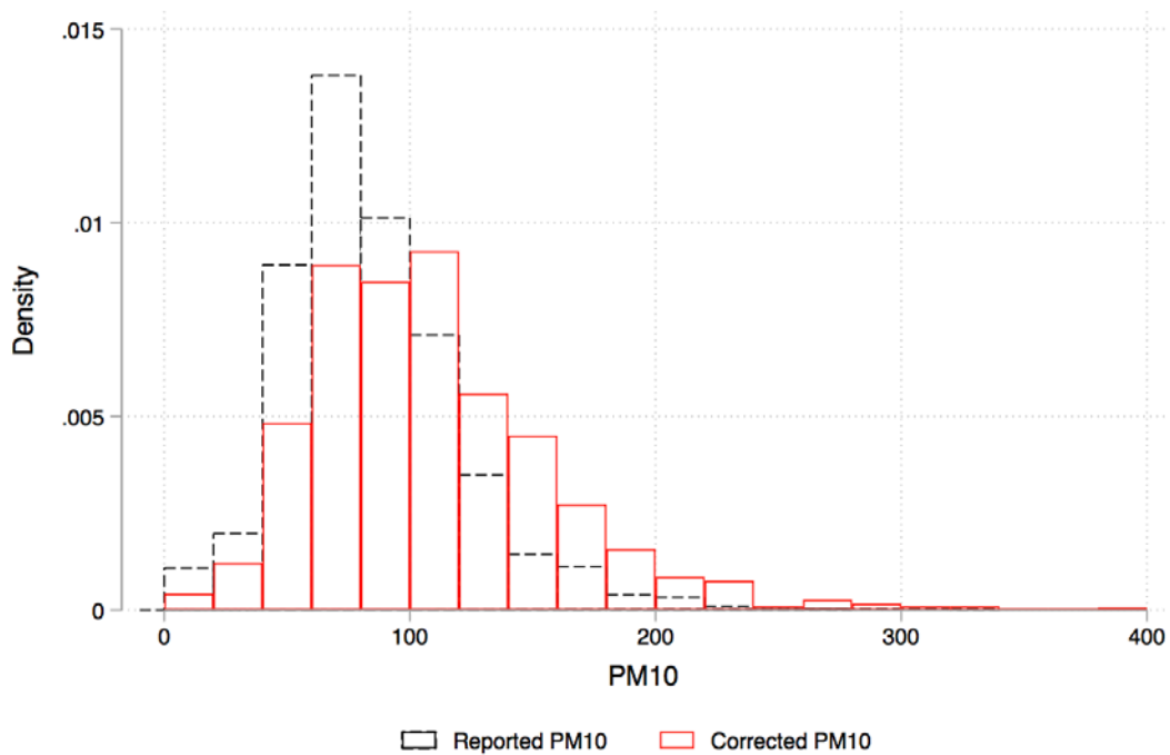
Figure B10. Correction of Pre-Automation PM 10 Data
