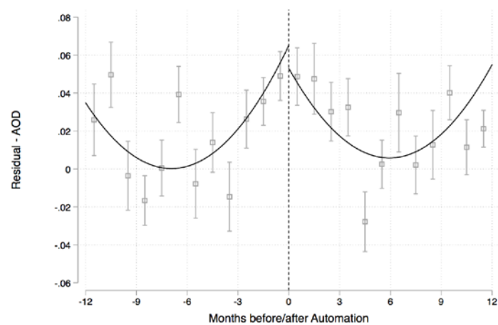
(B). Monthly Residual AOD
