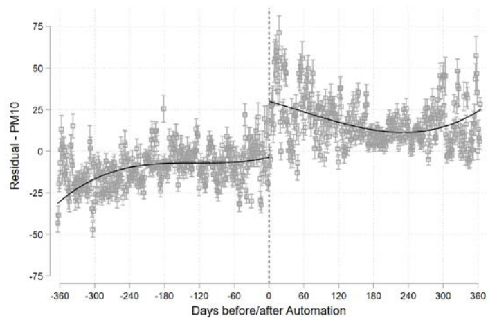
(A). Daily Residual PM 10
